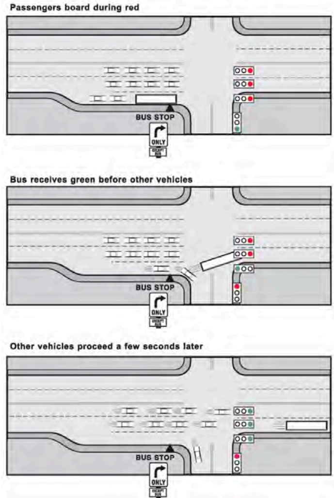
Bus Queue Jump Illustration
